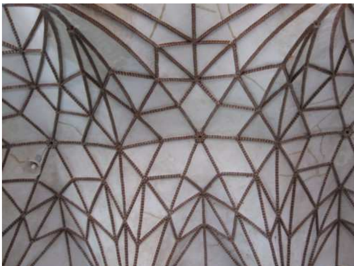
6. Intricate layout of gothic vaults
